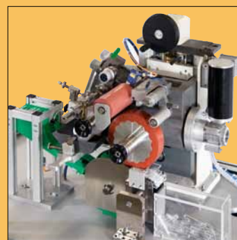
HSC-COMPACT automation Rotary pad printing
