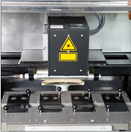
Linear motor axis with receiver plate for 4-colour screen set
